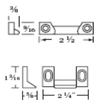
Strike for Rim Device Floor and stop strike for VR Device
