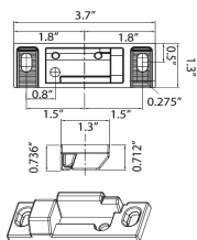
Strike for Rim Device Floor and stop strike for VR Device
